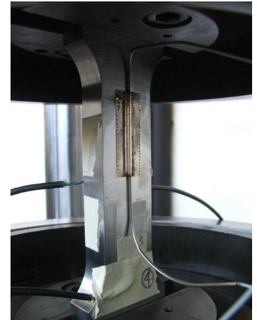
SmartWeld undergoing calibration and fatigue testing at UKAS accredited testhouse
